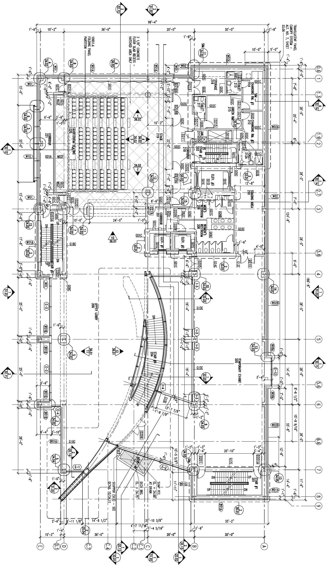
1 SECOND FLOOR PLAN SCALE: 1/8" = 1'-0" 0 2' 4' 8' 16' SECOND FLOOR GROSS AREA: 13,498 sqft. SECOND FLOOR NET AREA: 11,472 sqft.
